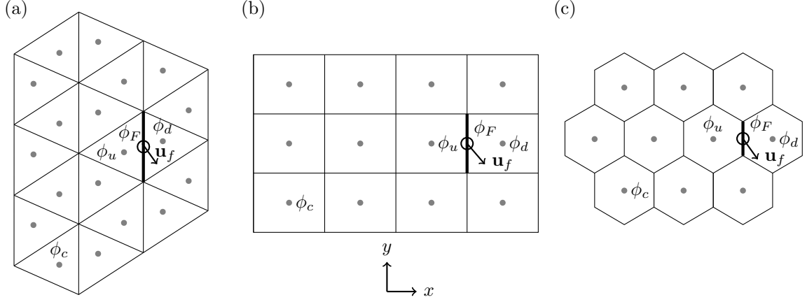
Figure 1: Upwind-biased stencils for faces far from the boundaries of two-dimensional (a) triangular, (b) rectangular and (c) hexagon meshes. The stencil is used to fit a multidimensional polynomial to cell centre values, \phi_c , marked by grey circles, in order to approximate the value \phi_F at the face centroid marked by an open circle. \phi_u and \phi_d are the values at the centroids of the upwind and downwind cells neighbouring the target face, drawn with a heavy line. The wind vector \mathbf{u}_f is prescribed at face f and determines the choice of stencil at each timestep.
