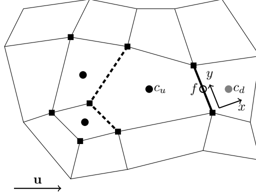
Figure 2: A thirteen-cell, upwind-biased stencil for face f connecting the pentagonal upwind cell c_u , and the downwind cell c_d . The dashed lines denote the two faces of cell c_u that oppose f , and black circles mark the centroids of the internal cells that are connected to these two opposing faces. The stencil is extended outwards by including cells that share vertices with the three internal cells, where black squares mark these vertices. The local coordinate system (x, y) has its origin at the centroid of face f , marked by an open circle, with x normal to f and y perpendicular to x .
